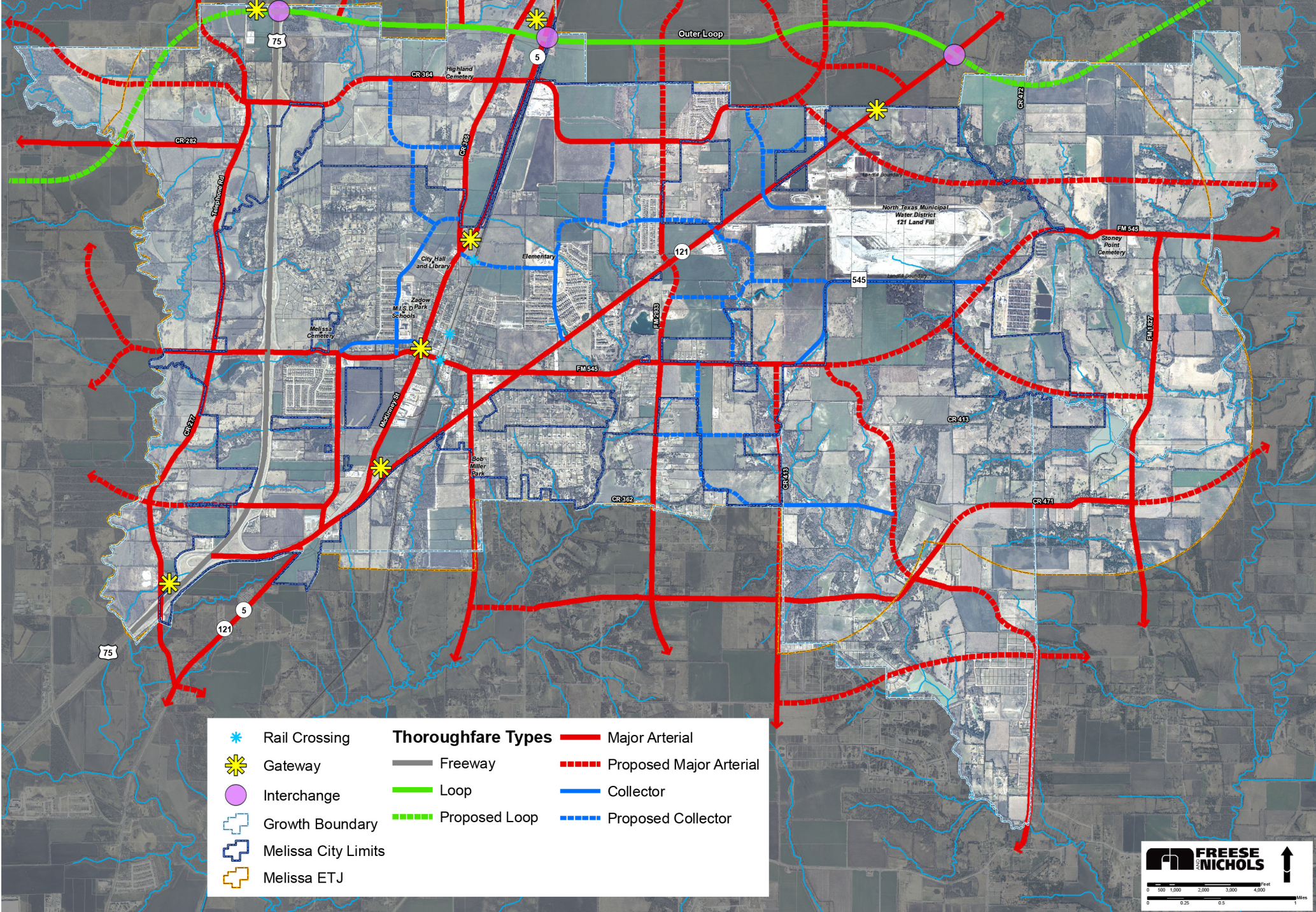
Figure 5-8. Transportation Plan Map
